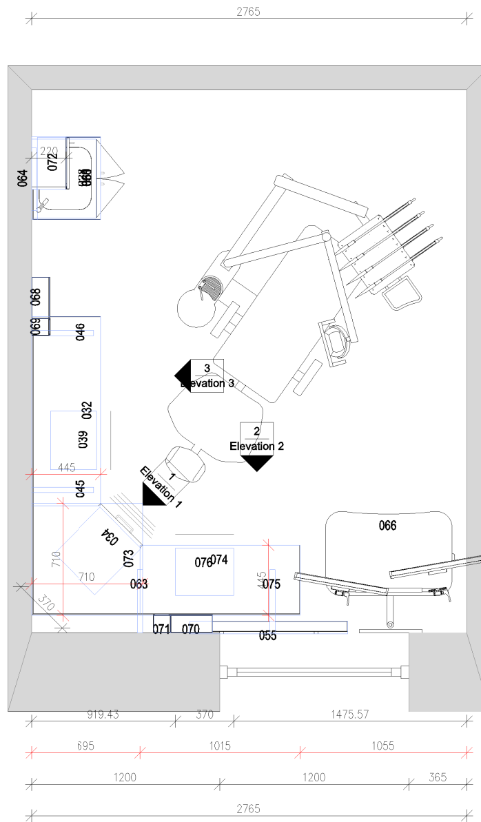
Plan view 1
